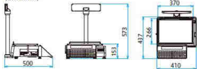
Uni-3 L2-Pole Model
