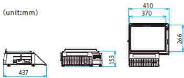
Uni-3 L1 B Model
